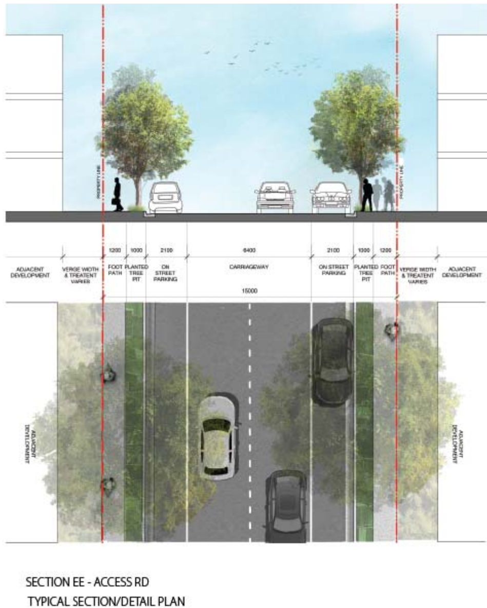
Figure 9 Street section EE – Access Road
